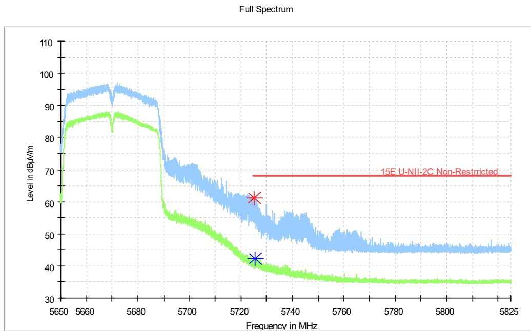
Fig. 15 Band Edges (802.11n-HT40 Ch134, 5670MHz)
