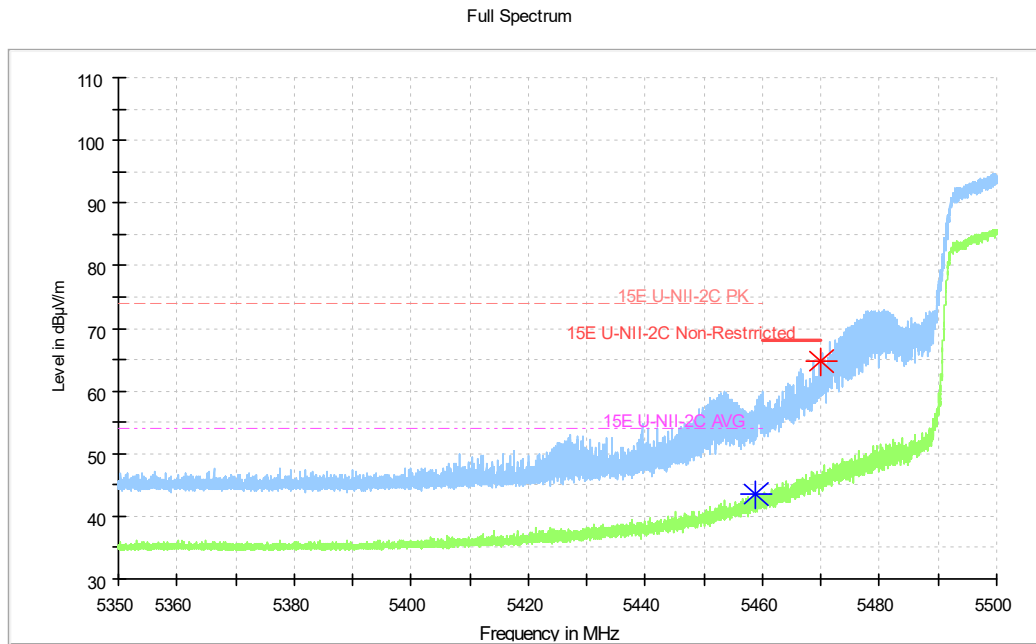
Fig. 14 Band Edges (802.11n-HT40 Ch102, 5510MHz)
