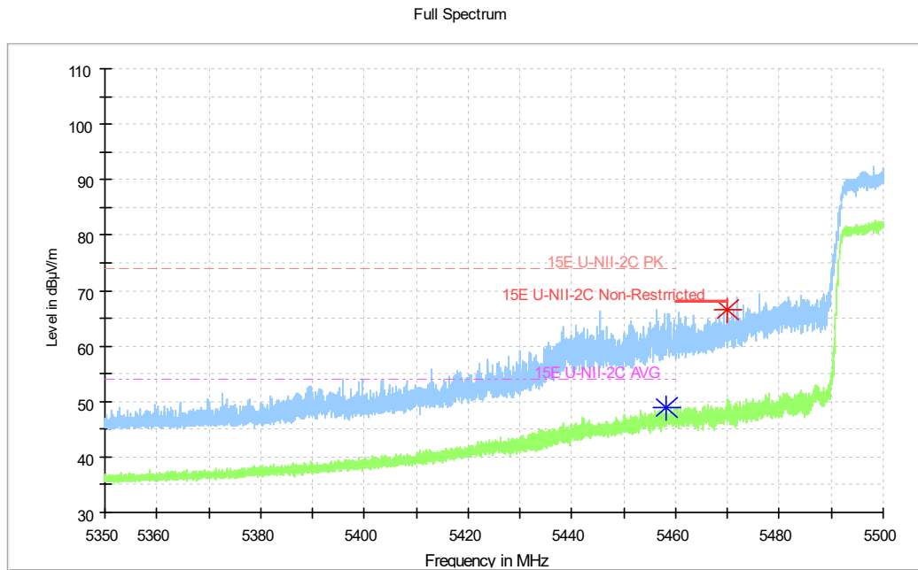
Fig. 26 Band Edges (802.11ac-HT80 Ch106, 5530MHz)
