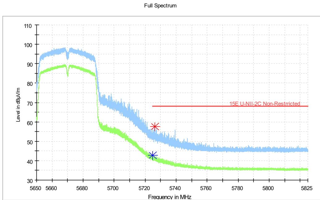
Fig. 23 Band Edges (802.11ac-HT40 Ch134, 5670MHz)
