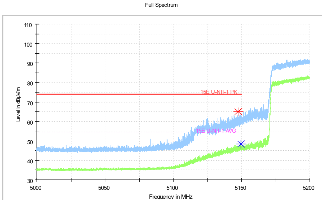
Fig. 24 Band Edges (802.11ac-HT80 Ch42 , 5210MHz)
