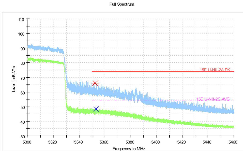
Fig. 25 Band Edges (802.11ac-HT80 Ch58, 5290MHz)
