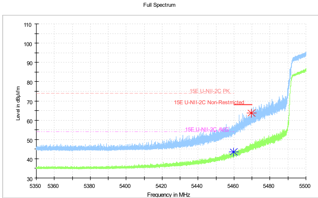
Fig. 22 Band Edges (802.11ac-HT40 Ch102, 5510MHz)
