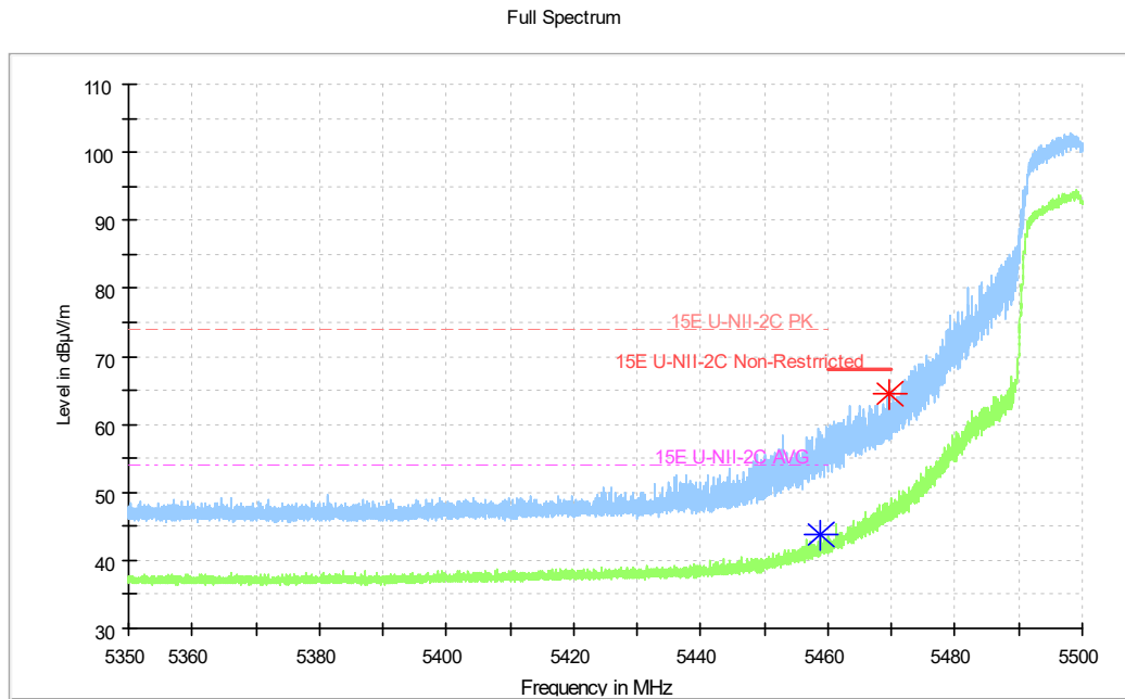
Fig. 10 Band Edges (802.11n-HT20 Ch100, 5500MHz)
