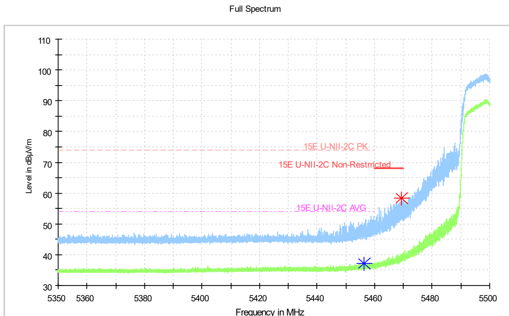
Fig. 18 Band Edges (802.11ac-HT20 Ch100, 5500MHz)
