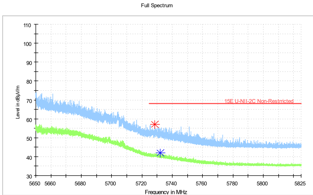
Fig. 27 Band Edges (802.11ac-HT80 Ch122, 5610MHz)
