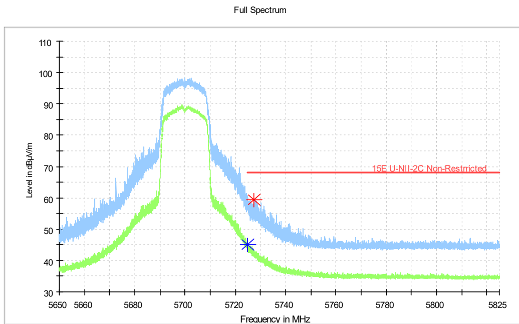
Fig. 19 Band Edges (802.11ac-HT20 Ch140, 5700MHz)
