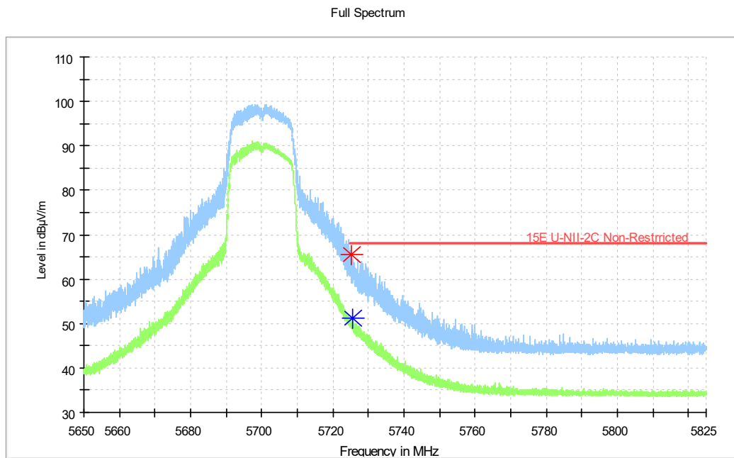
Fig. 11 Band Edges (802.11n-HT20 Ch140, 5700MHz)
